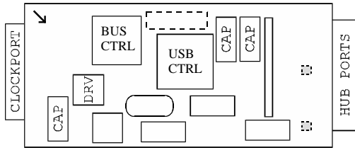
[Fig. 1] Connectors on the SUBWAY. (top side view)
