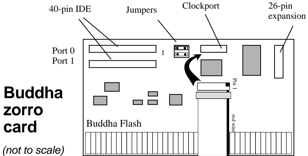
[Fig. 2] Cable connection scheme (top side view)
